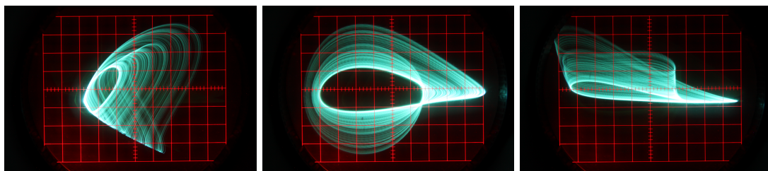
Figure 3: Phase space plots of the chaotic system with one stable equilibrium
