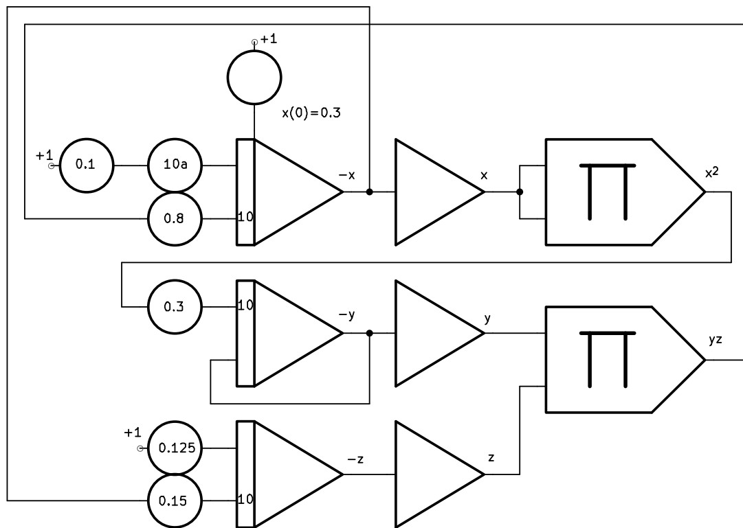
Figure 1: Analog computer program of the chaotic system with one stable equilibrium
