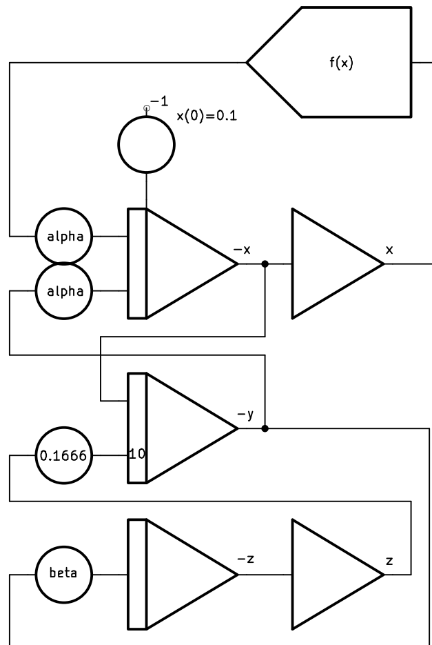
Figure 6: Circuit implementing equations (5), (6), and (7)
