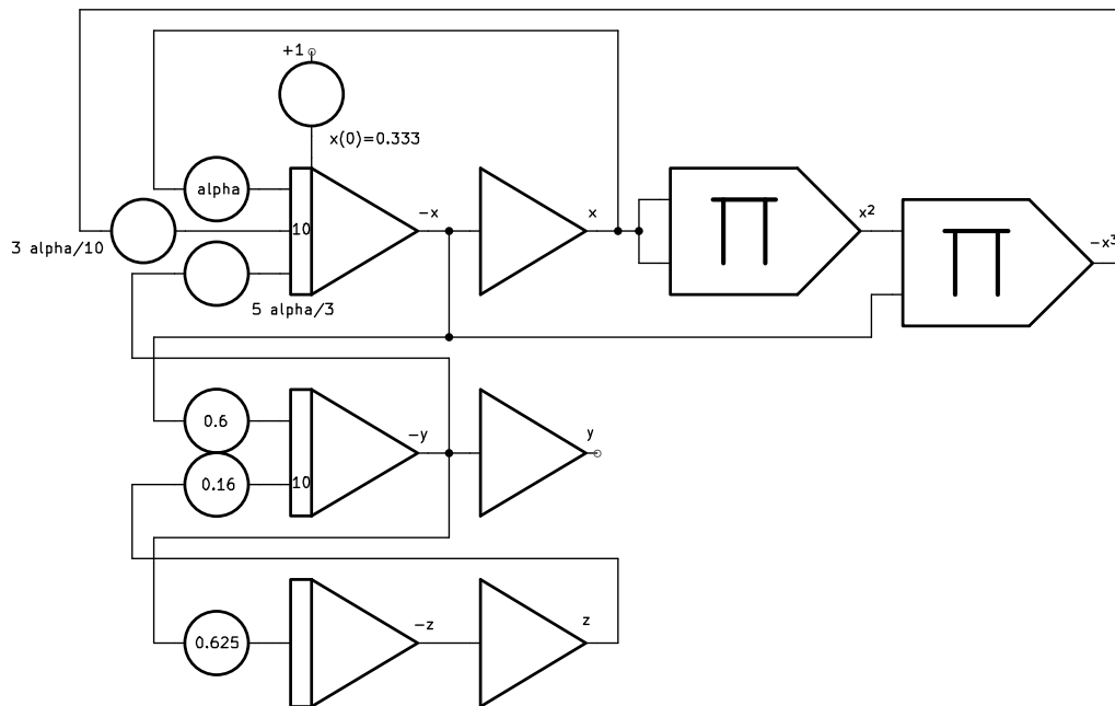
Figure 10: Analog computer program for the cubic system
