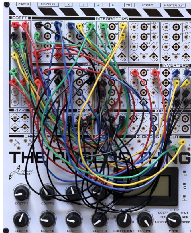
Figure 8: Actual implementation of the circuits shown in figures 6 and 7
