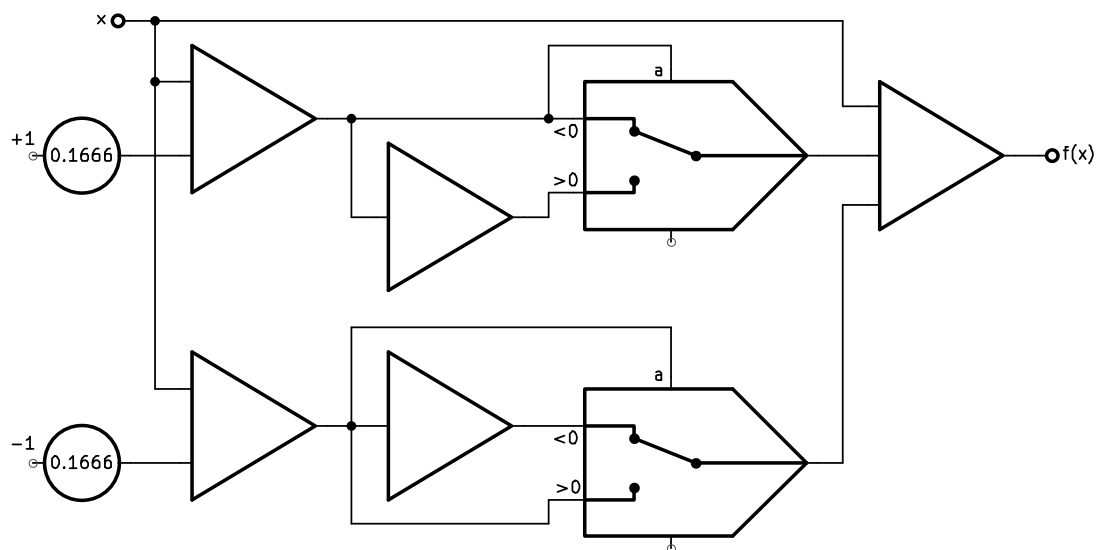
Figure 7: Circuit implementing equation (8)
