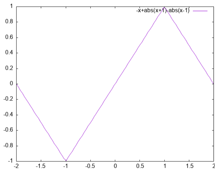
Figure 4: f(x) for x \in [-2, 2]
