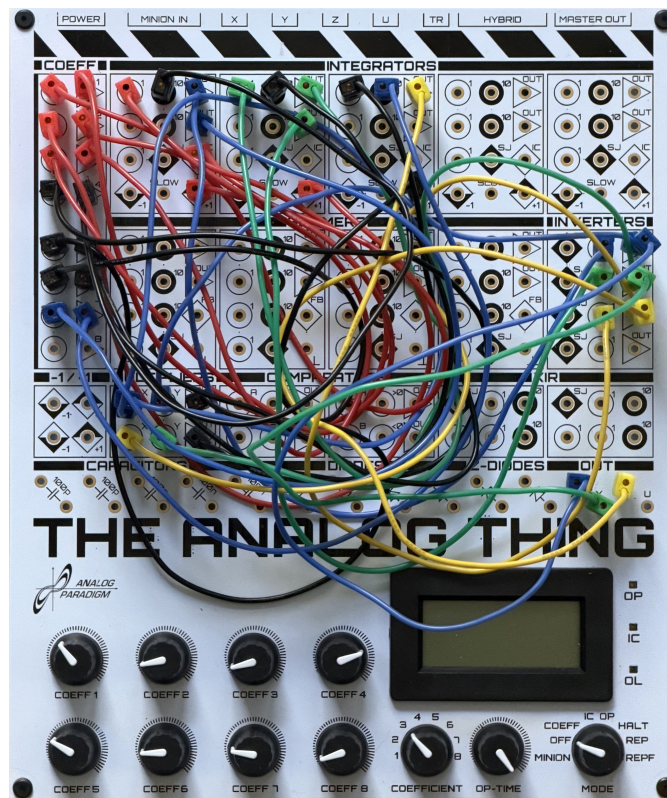
Figure 2: Implementation of the chaotic system with one stable equilibrium on THE ANALOG THING
