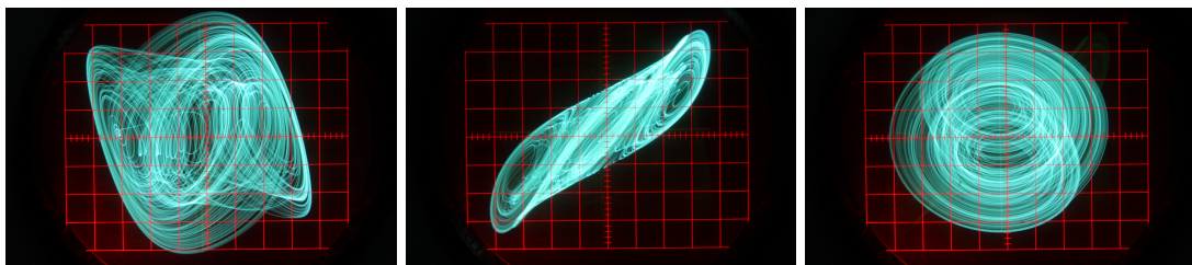
Figure 12: Double-scroll-attractor of the cubic system
