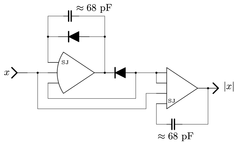
Figure 5: Standard circuit for an absolute value function
