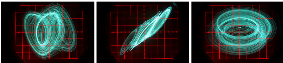
Figure 9: Double-scroll-attractor of the GMC-system
